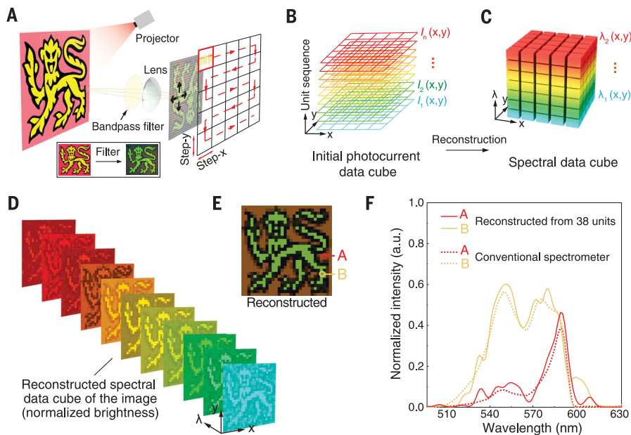
Fig. 3. Scanning spectral imaging at the macroscale. (A) Schematic of spectral imaging by our nanowire spectrometer. A bandpass filter is used to remove signals outside the detectable range of the spectrometer. Spectral imaging is conducted by scanning the nanowire spectrometer on the focal plane in a serpentine pattern. (B) Each pixel contains a photocurrent value from each photodetector unit, forming an initial data cube. (C) A spectral data cube is computationally reconstructed from the photocurrent data cube. (D) A series of reconstructed images at selected wavelengths. The intensity range of these images is normalized. (E) Pseudo-colored spectral image converted from the spectra according to CIE color matching functions. (F) Spectra of points A and B in (E), measured by a nanowire spectrometer and a conventional spectrometer.
